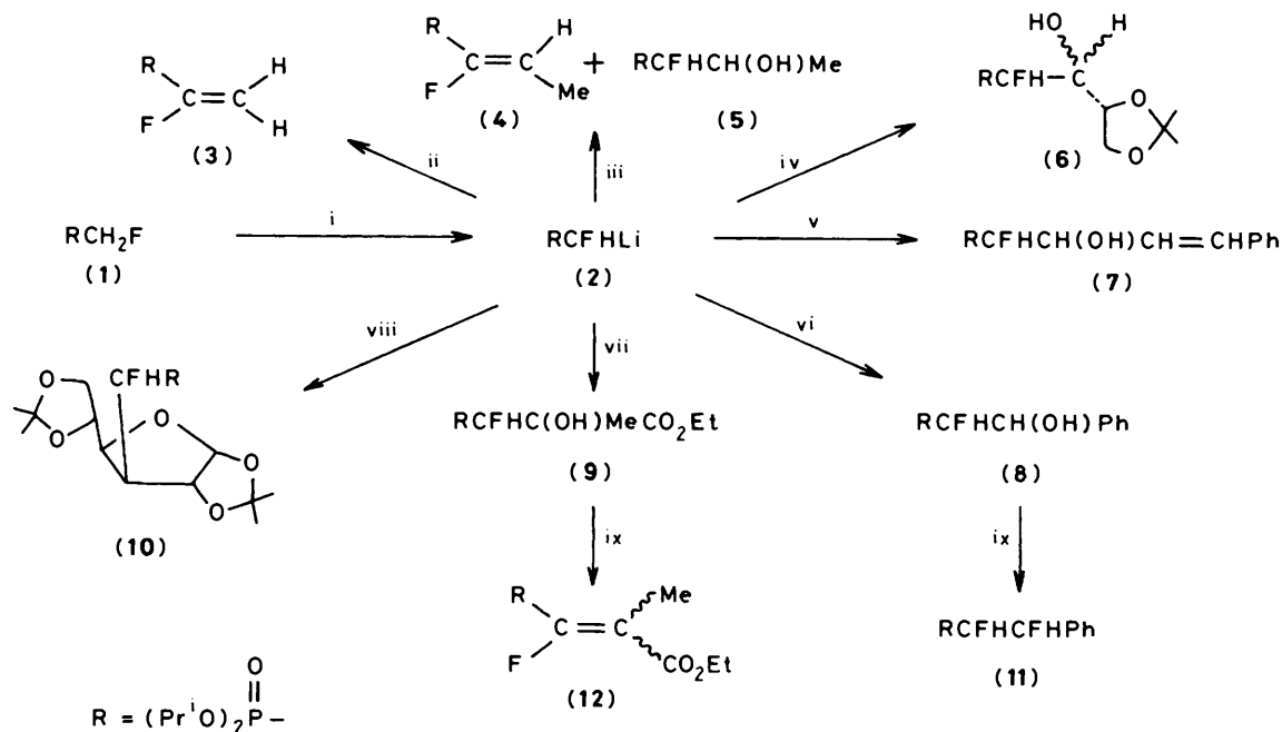
Scheme 1. Reagents: i, LDA–THF, -78^\circ C ; ii, (CH_2O)_n ; iii, MeCHO; iv, RCH_2OCMe_2OCHCHO ; v, PhCH=CHCHO ; vi, PhCHO; vii, MeCOCO 2 Et; viii, 1,2:5,6-di- O -isopropylidene- \alpha - D -ribo-hexofuran-3-ulose; ix, DAST.
